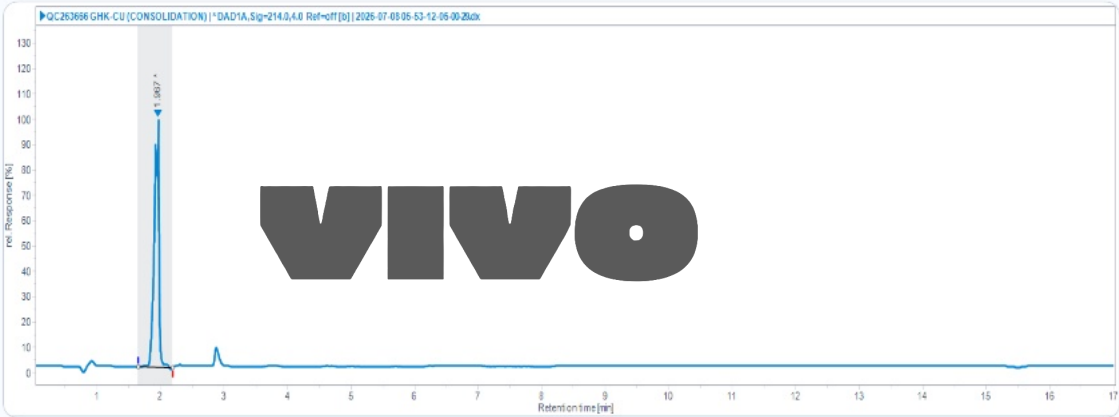
HPLC Chromatogram (Retention Time: 1.967 min)
