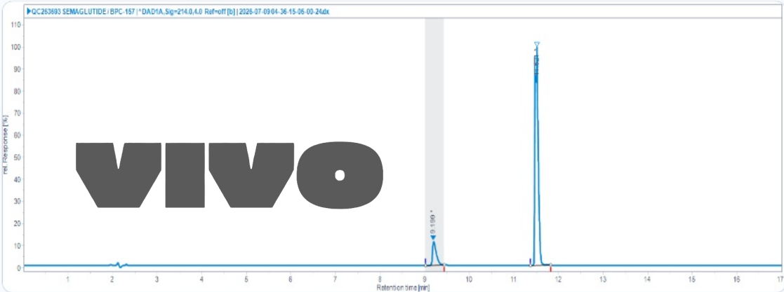
HPLC Chromatogram (Retention Time: 9.199, 11.521 min)
