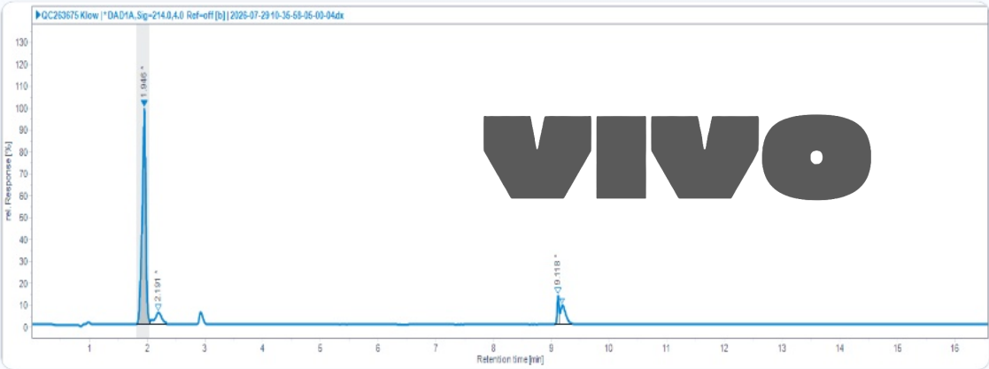
HPLC Chromatogram (Retention Time: 1.946, 2.191, 9.118, 9.195 min)
